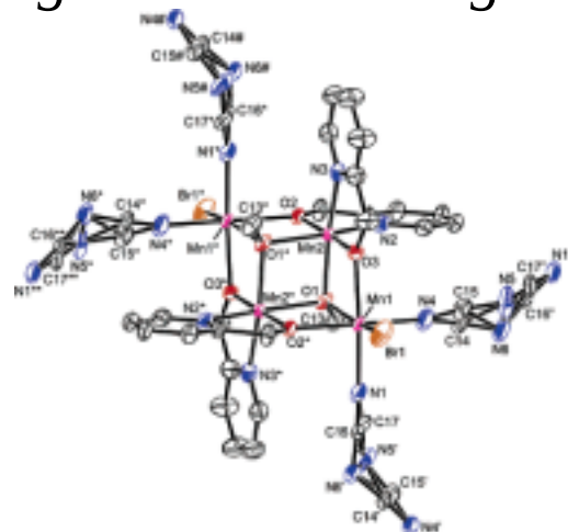
Single Molecule-Magnet
