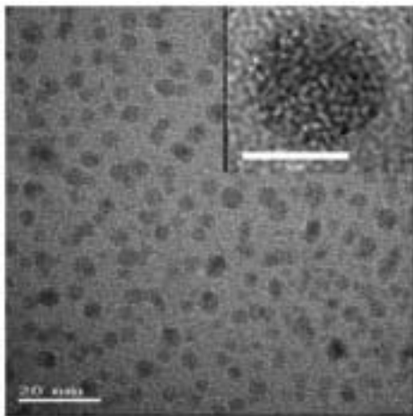
Magnetic Nano-Particle
